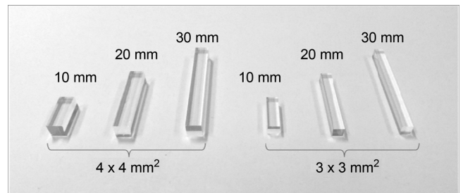
Fig. 9. Various sizes of LYSO crystals used in this study, all surfaces of which were mechanically polished.
