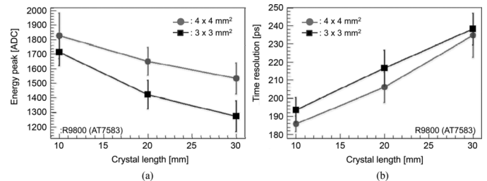
Fig. 10. (a) Light output and (b) Time resolution as a function of the crystal length and cross-section.
