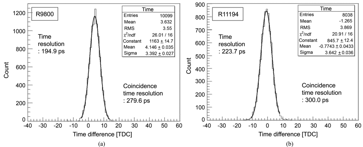
Fig. 4. Timing performance measured by fast PMTs with a LYSO crystal ( 4 \times 4 \times 10 mm) in the optimal time discrimination setup. Coincidence time difference distributions were obtained by using (a) R9800 and (b) R11194 PMTs.
