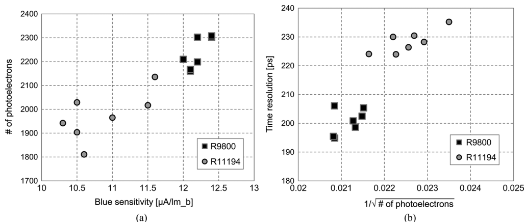
Fig. 6. The effect of the number of photoelectrons, and the blue sensitivity of individual PMTs on the time resolution (a) The number of photoelectrons emitted from the photocathode in the PMT against the blue sensitivity of the individual PMTs and (b) The correlation of time resolution with the number of photoelectrons.
